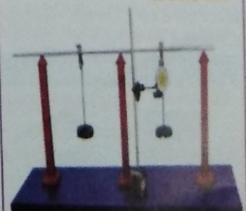
DEFLECTION OF TRUSS APPARATUS
